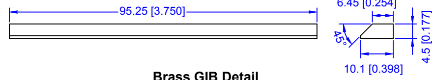
Brass GIB Detail
